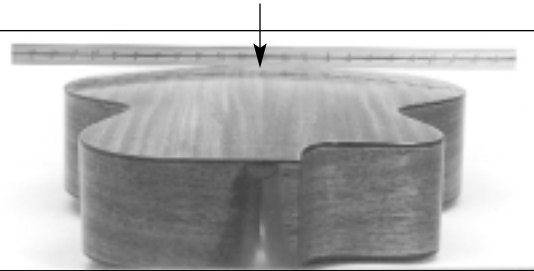
Photo 1. This photo shows an extremely swollen guitar back. Notice the dip in the center, where the back is glued to the tailblock. It cannot rise at this section and so a ripple, or low spot, is created.
