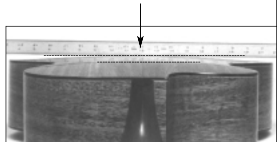
Photo 6. This photo shows the back arch after the guitar has been dried. Notice that the swelling on the back is less pronounced. This guitar lost 38 grams of weight in the drying process, which translates into 1-1/3 ounces of water!
