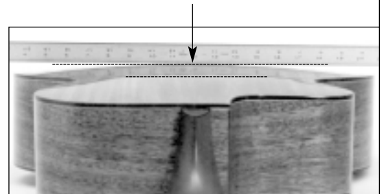
Photo 5. This photo shows a back arch that is very high from excess moisture.
