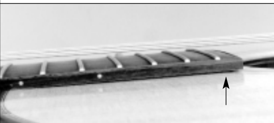
Photo 3. This photo shows the top and fretboard swollen so much that the glue joint has failed and the two pieces have popped apart.
